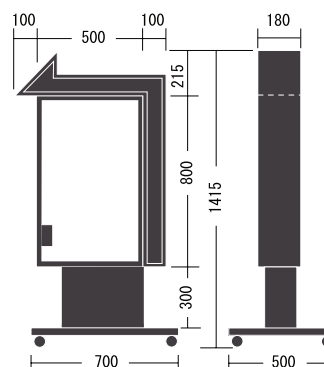
FX-850LED
