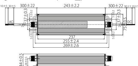
●A1PS-H398C150 (150W 型)
