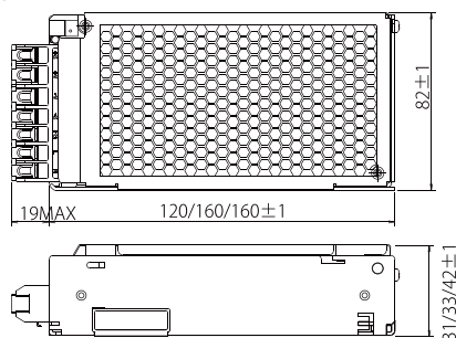
●HWS50A/100A/150A
